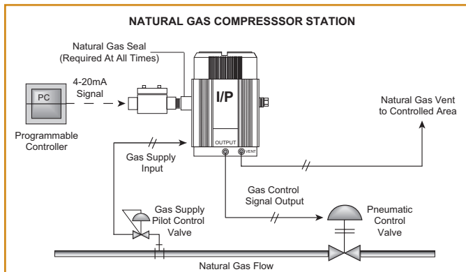
Figure 1. The IPX 2 Current-to-Pressure Transmitter provides an interface between electronic control systems, such as a DCS or PLC or RTU and a pneumatic control valve actuator.
