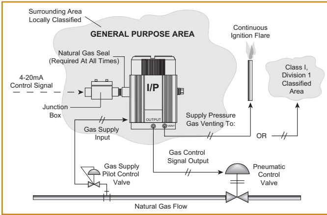
APPLICATION #1—Explosion-Proof Installation in General Areas*
