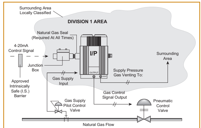
APPLICATION #6—Intrinsically-Safe Installation in Division 1 and Zone 0 Areas*
