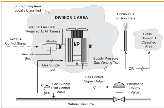
APPLICATION #2—Explosion-Proof Installation in Division 2 Areas*
