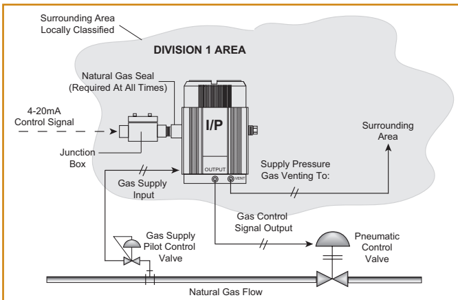
APPLICATION #3—Explosion-Proof Installation in Division 1 Areas*
